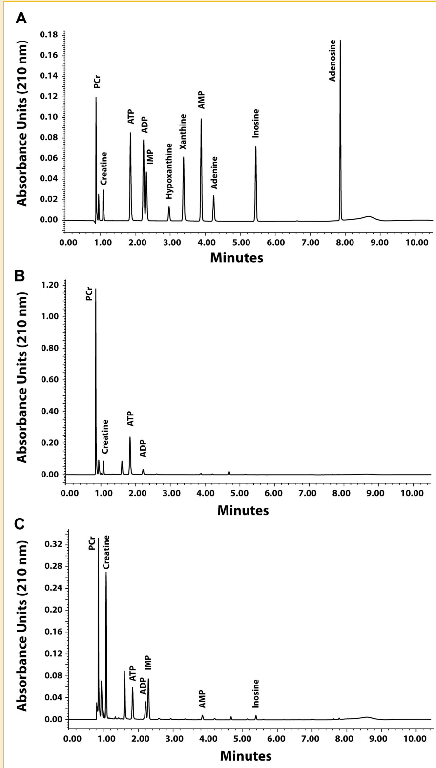
Fig. 1. Ultra-performance liquid chromatography chromatograms. A: Chromatogram of a standard mixture containing 100 pmol each phosphocreatine (PCr), creatine, ATP, ADP, AMP, IMP, adenosine, inosine, and xanthine and 25 pmol each hypoxanthine and adenine. Detection limits are less than 1.0 pmol. B: Chromatogram of a perchloric acid extract of a non-contracted EDL muscle incubated at resting length. Injection volume was 2 \mu l. C: Chromatogram of an extract from an EDL muscle after contracting at 10 Hz for 15 min.
