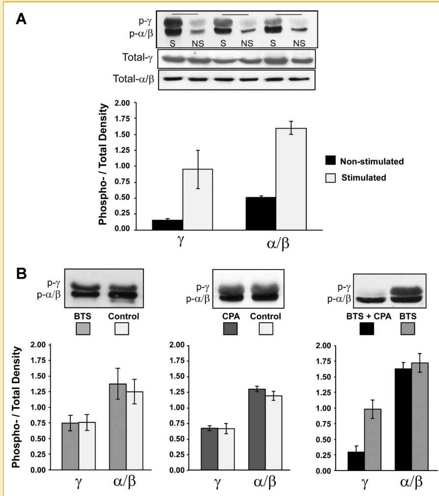
Fig. 5. The increase in phosphorylation of p38-MAPK isoforms in skeletal muscle with electrical stimulation is prevented by combined treatment with BTS and CPA. A: Muscles were either stimulated (S) at 10 Hz for 15 min, or non-stimulated (NS). Protein levels of phospho-p38 MAPK isoforms and total p38 MAPK were determined by Western blot. Quantification was based on the fraction of phosphorylated protein relative to the total detected by Western blot analysis ( n = 3 ). B: Muscles were treated without (control) or with (BTS and CPA) cytosolic ATPase inhibitors and then stimulated for 15 min. Protein levels of phospho-p38 MAPK isoforms were determined by Western blot. Bar graphs represent the mean \pm SE; n = 4 .
