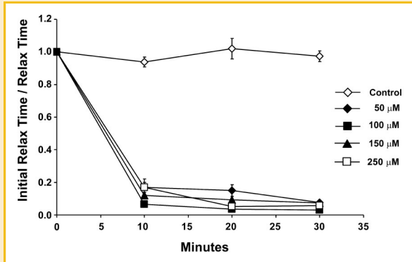
Fig. 2. Dose response curves for cyclopiazonic acid (CPA) over time in isolated EDL mouse muscles. Inhibition of SERCA by CPA was evaluated by measuring the total relaxation time for each twitch contraction (in ms), normalized to the percent of initial (Time 0), and then expressed as the reciprocal. The data are presented as mean \pm SE.
